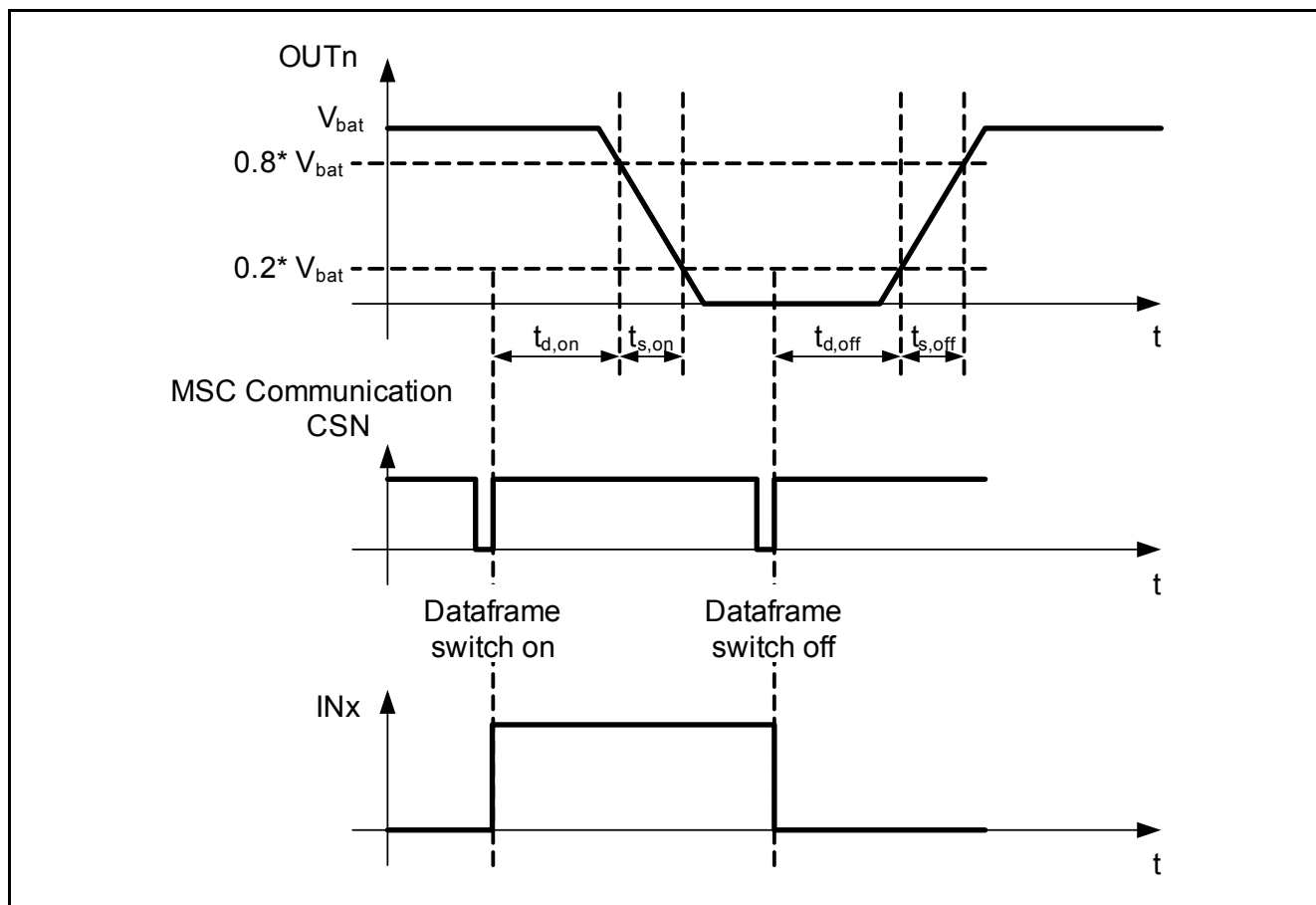
Figure 31 Switching Behavior
