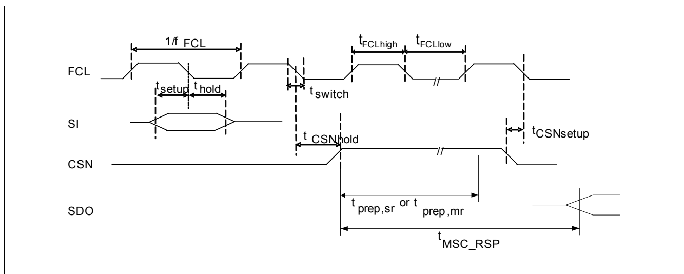
Figure 63 MSC timing
