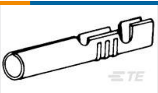
TE Part #42827-2 PIN .093 RECEPTACLE 24-18 AWG TPBR
