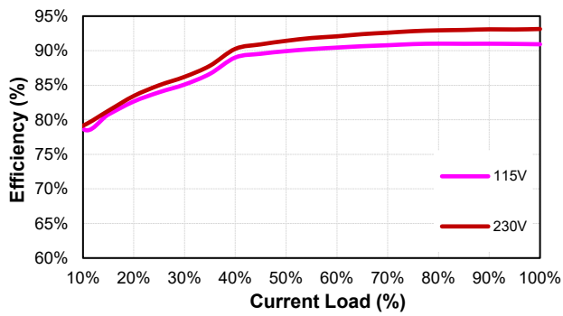
CFM150S120 (Eff Vs Io)
