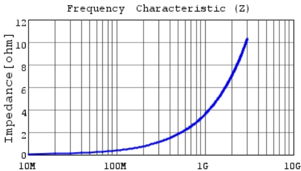
LQP02TQ0N6C02 |Z|
