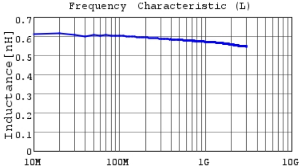
LQP02TQ0N6C02 L
