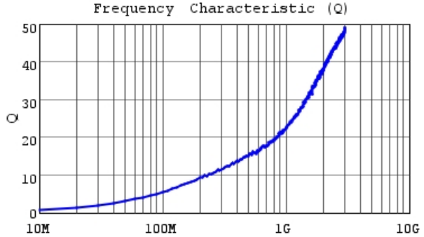
LQP02TQ0N6C02 Q
