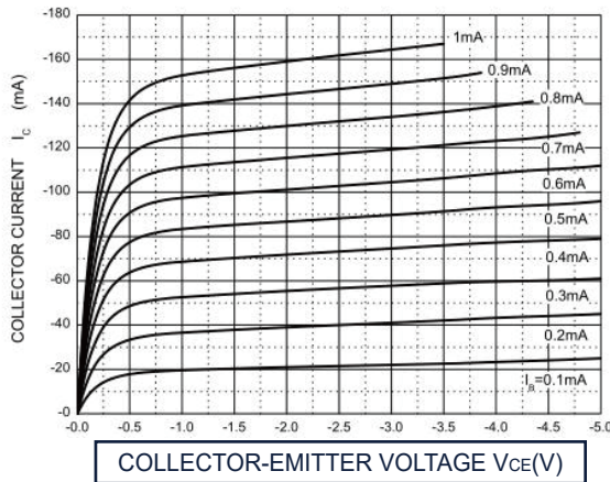
Static Characteristic
