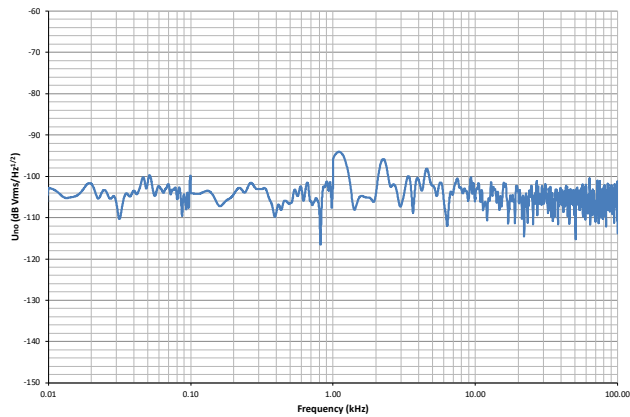
Figure 10: Typical output noise voltage spectral density U_{no} referred to secondary
