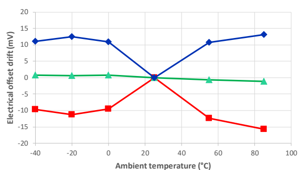
Figure 3: Electrical offset thermal drift
