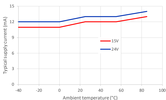
Figure 1: Supply current function of temperature
