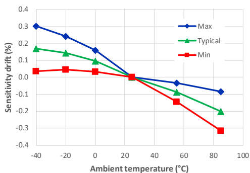
Figure 4: Sensitivity thermal drift
