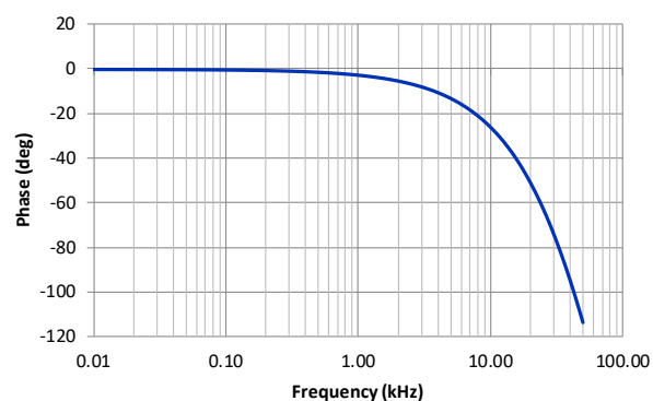
Figure 9: Phase shift function of frequency
