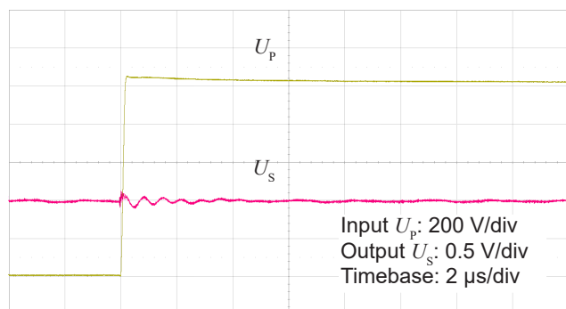
Figure 6: Detail of typical common mode perturbation (1000 V step with 6 kV/ \mu s)
