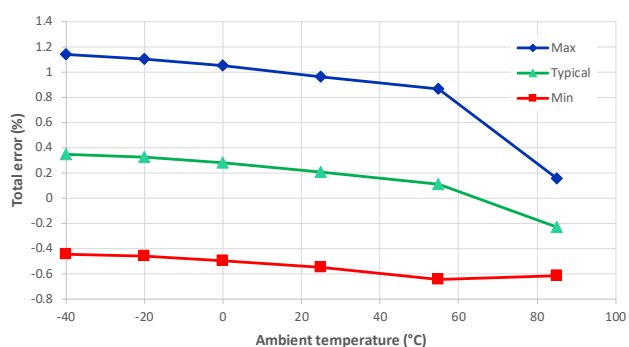
Figure 2: Total error in temperature
