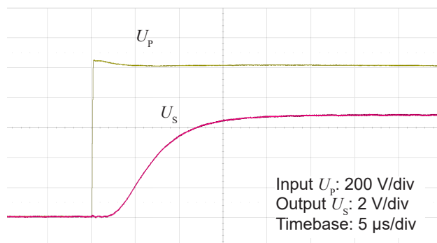
Figure 7: Typical step response (0 to 1000 V)
