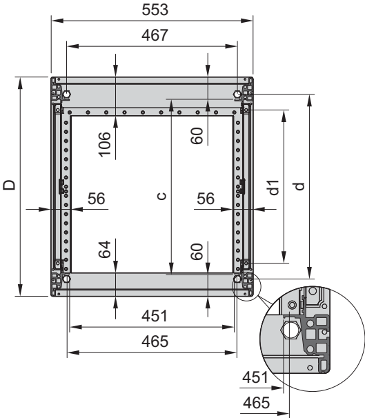
Frame (top view)
