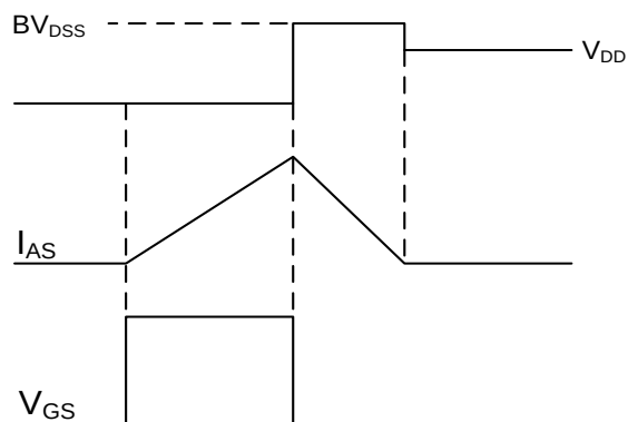
Fig.11 EAS Waveform
