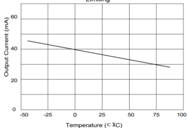
Fig.11 Current Limiting
