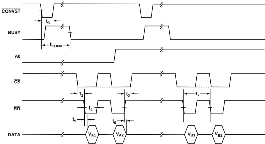
Figure 1. Timing Diagram
