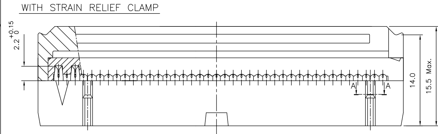
CABLE DIMENSIONS
