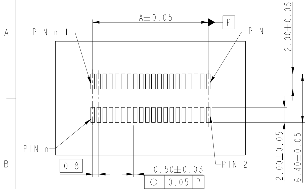
RECOMMENDED PCB LAYOUT WITHOUT PEGS AND HOLDDOWN
