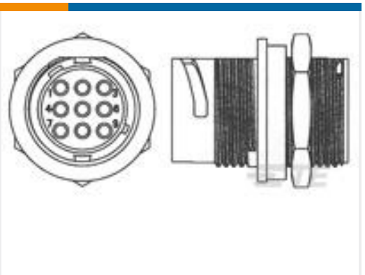
TE Part #1445821-3 REC,11-8,FLNG MT,LG INS,STD KE
