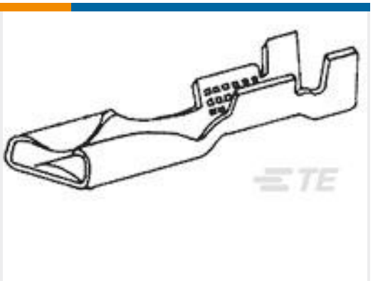
TE Part #60435-1 FF 187 REC 20-16AWG PTBR
