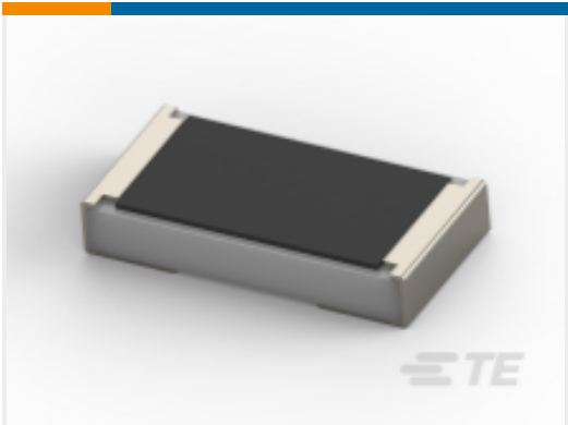
TE Part #2-2176231-5 SMD Power Resistor: 3 Watt, 1% Tol
