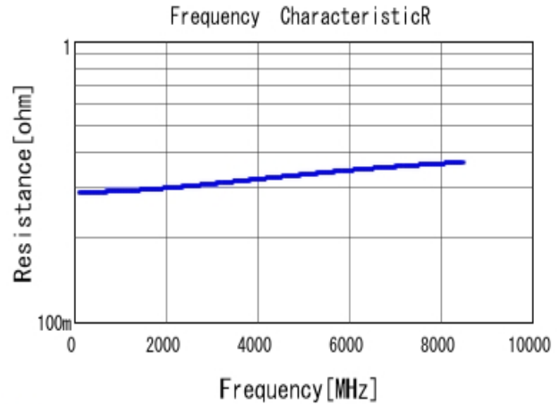
■ GJM0335C1E1R1BB01 R DC0V, 25degC
