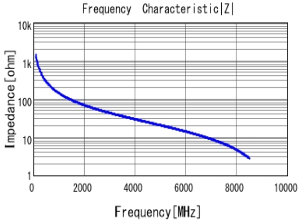
■ GJM0335C1E1R1BB01 |Z| DC0V, 25degC
