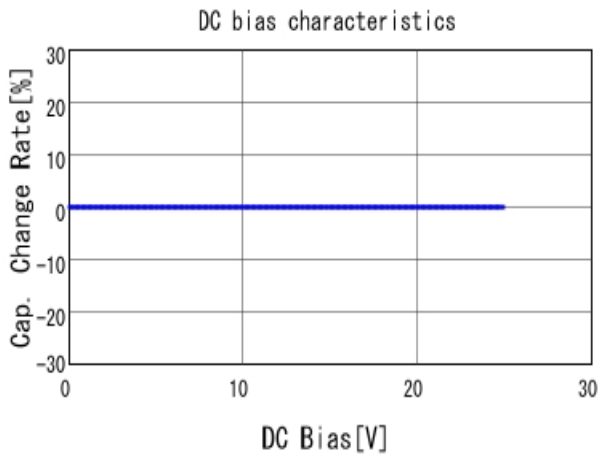
■ GJM0335C1E1R1BB01 C-DC bias capchange, 25.0degC, AC1V
