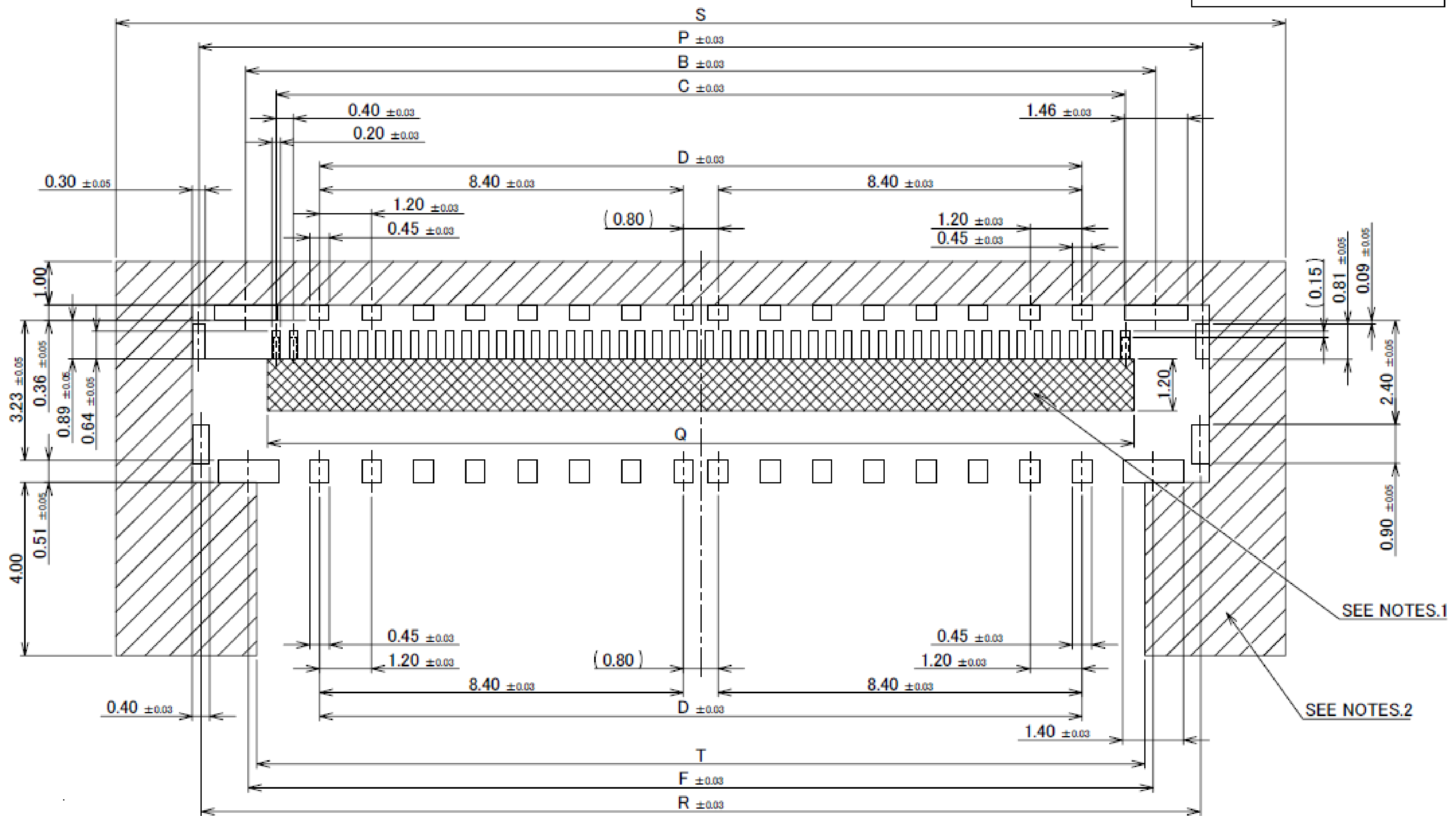
#1 TYPE 50P RECOMMENDED PCB LAYOUT (S=10/1)
