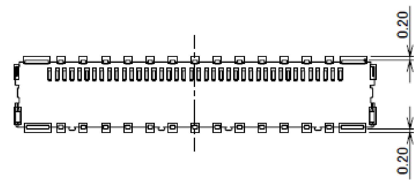
CONNECTOR ON RECOMMENDED FOOTPRINT PATTERN ※#1 TYPE
