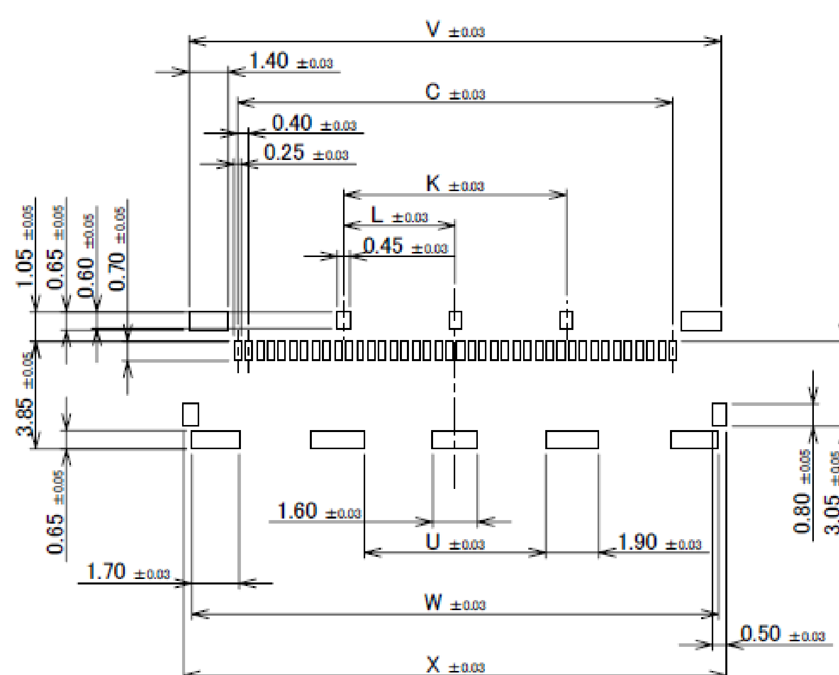
02 TYPE 40P RECOMMENDED METAL MASK LAYOUT (S = 5 : 1) ※ METAL MASK THICKNESS : t = 0.12
