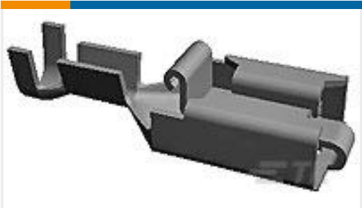
TE Part #927854-1 PL 250 REC TERMINAL 17-13 AWG BR
