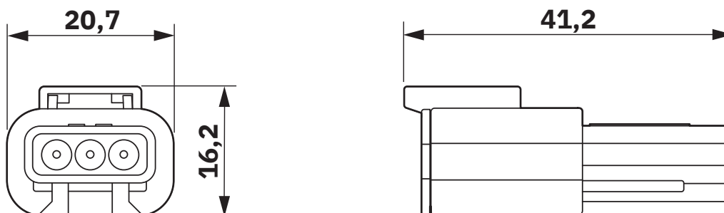
ATM04-3P top view and side view
