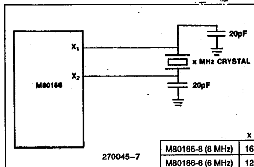
Figure 8. Recommended M80186 Crystal Configuration
