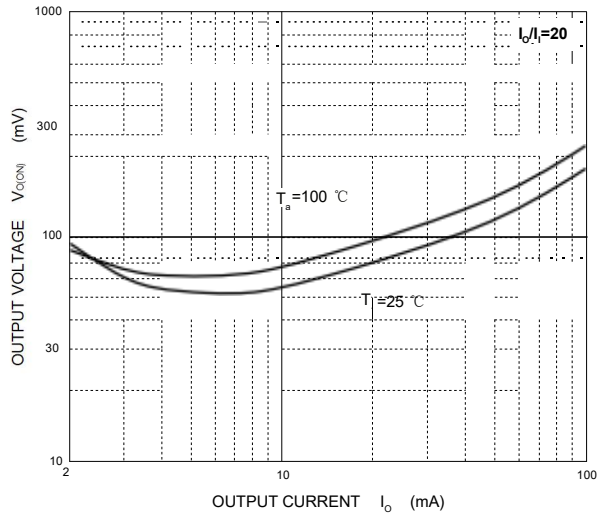
V_{O(ON)} — I_O
