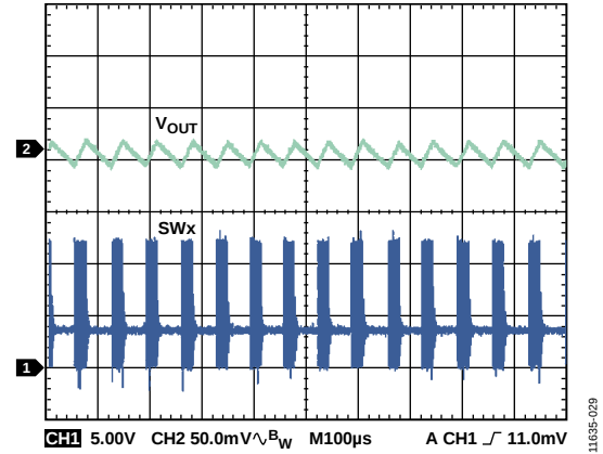
Figure 26. Steady State Waveform at Light Load, V_{IN} = 12\text{ V} , V_{OUT} = 3.3\text{ V} , I_{OUT} = 30\text{ mA} , f_{SW} = 600\text{ kHz} , L = 4.7\text{ μH} , C_{OUT} = 47\text{ μF} \times 2 , Automatic PWM/PSM Mode
