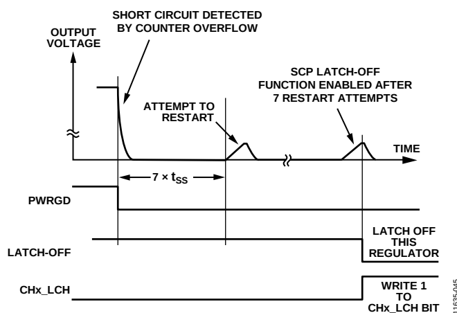
Figure 47. Short-Circuit Latch-Off Detection
