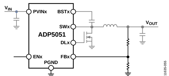
Figure 62. Typical Circuit with High Current Traces Shown in Gray
