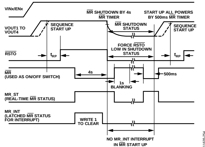
Figure 54. \overline{\text{MR}} Timing Diagram in Power-On/Off Switch Mode
