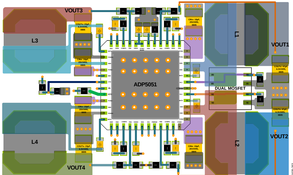
Figure 63. Typical PCB Layout
