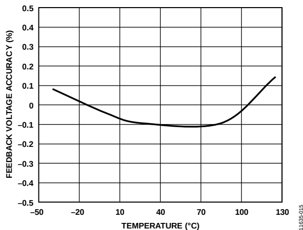
Figure 17. 0.8 V Feedback Voltage Accuracy vs. Temperature for Channel 1, Adjustable Output Model
