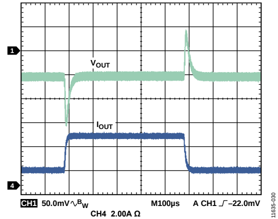
Figure 27. Channel 1/Channel 2 Load Transient, 1 A to 4 A, V_{IN} = 12\text{ V} , V_{OUT} = 3.3\text{ V} , f_{SW} = 600\text{ kHz} , L = 2.2\text{ μH} , C_{OUT} = 47\text{ μF} \times 2
