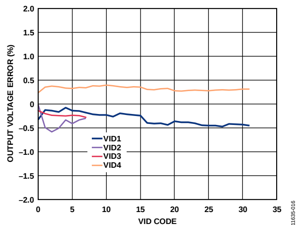
Figure 18. Output Voltage Error vs. VID Code, Adjustable Output Model
