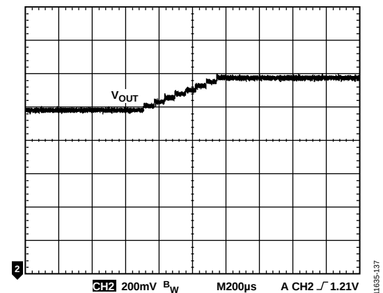
Figure 34. Channel 1 Dynamic Voltage Scaling (DVS) from 1.1 V to 1.3 V, 62.5 \mu s Interval, V_{IN} = 12\text{ V} , I_{OUT} = 4\text{ A} , f_{SW} = 600\text{ kHz} , L = 1\text{ }\mu\text{H} , C_{OUT} = 47\text{ }\mu\text{F} \times 2
