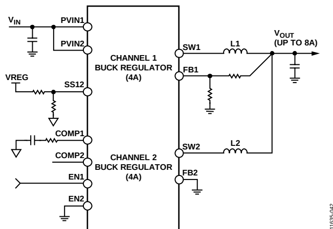
Figure 45. Parallel Operation for Channel 1 and Channel 2
