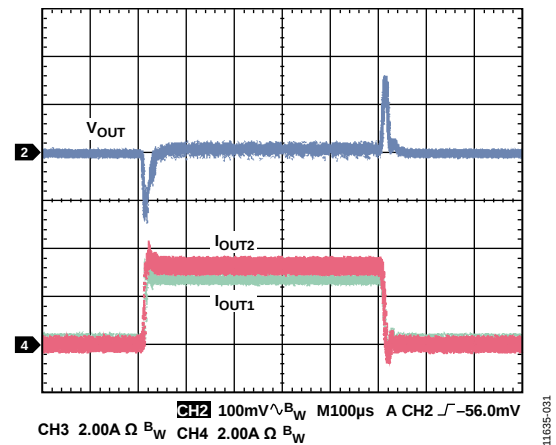
Figure 28. Load Transient, Channel 1/Channel 2 Parallel Output, 0 A to 6 A, V_{IN} = 12\text{ V} , V_{OUT} = 3.3\text{ V} , f_{SW} = 600\text{ kHz} , L = 4.7\text{ μH} , C_{OUT} = 47\text{ μF} \times 4
