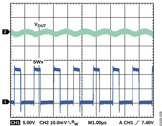
Figure 25. Steady State Waveform at Heavy Load, V_{IN} = 12\text{ V} , V_{OUT} = 3.3\text{ V} , I_{OUT} = 3\text{ A} , f_{SW} = 600\text{ kHz} , L = 4.7\text{ μH} , C_{OUT} = 47\text{ μF} \times 2 , FPWM Mode
