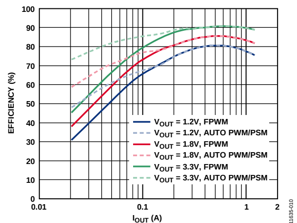
Figure 12. Channel 3/Channel 4 Efficiency Curve, V_{IN} = 12\text{ V} , f_{SW} = 600\text{ kHz} , FPWM and Automatic PWM/PSM Modes
