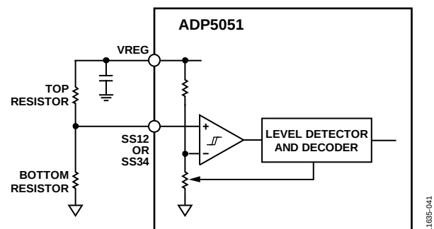
Figure 44. Level Detector Circuit for Soft Start
