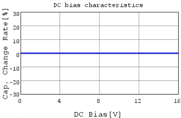
GRM0225C1C2R2CA03 C-DC bias capchange, 25.0C
