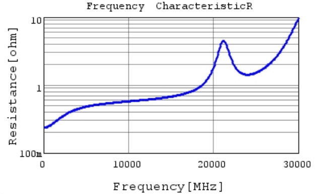
GRM0225C1C2R2CA03 R DCOV, 25degC
