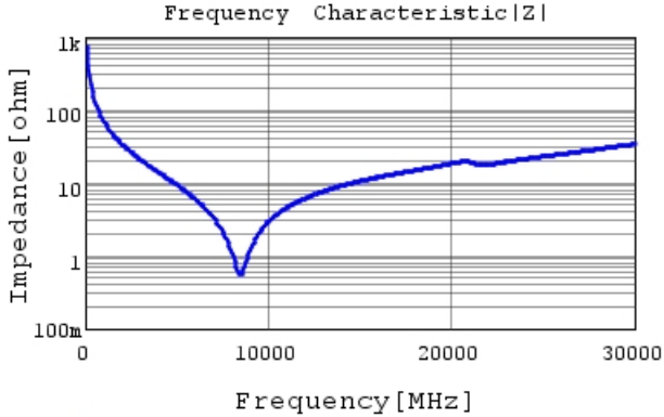
GRM0225C1C2R2CA03 |Z| DCOV, 25degC
