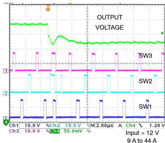
Figure 11. Load Transient
