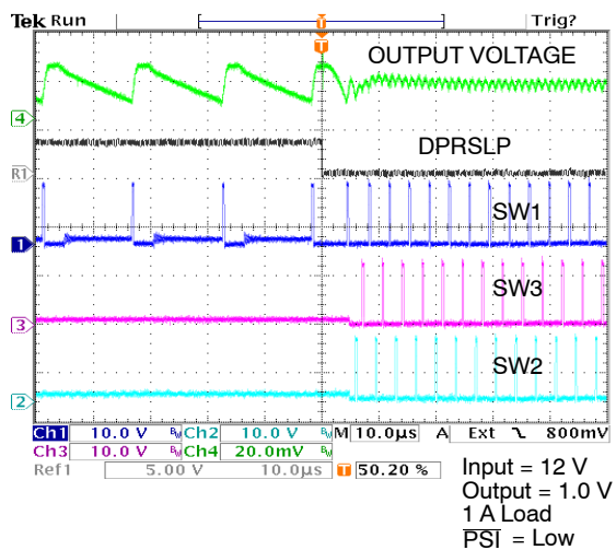
Figure 18. DPRSLP Transition
