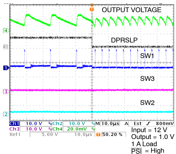
Figure 20. DPRSLP Transition
