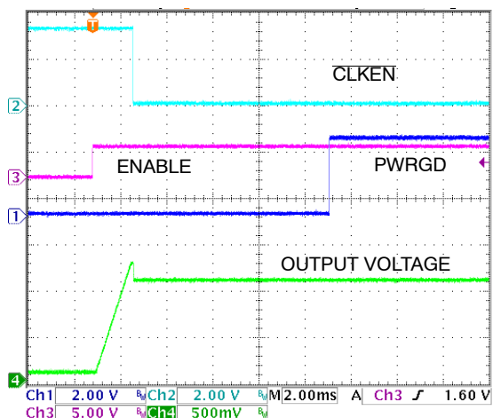
Figure 8. ADP3207C Startup
