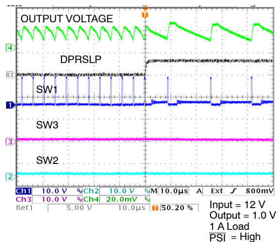
Figure 21. DPRSLP Transition
