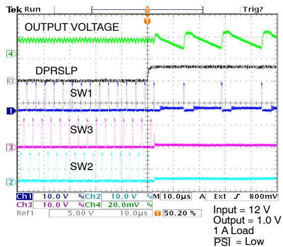
Figure 19. DPRSLP Transition
