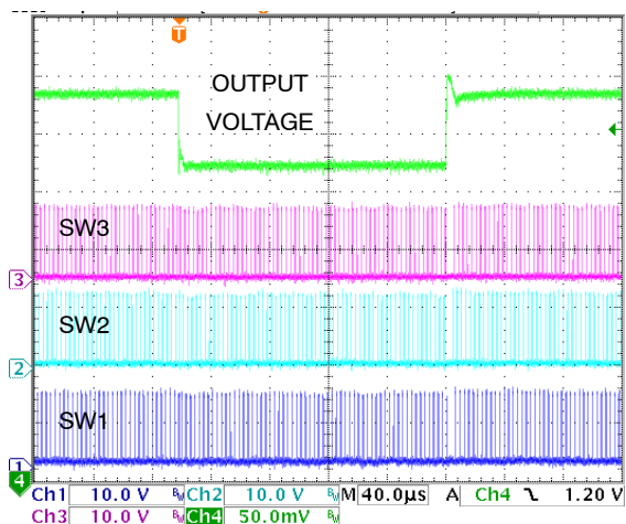
Figure 10. Load Transient
