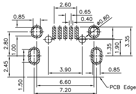
△ Recommended P.C.B. Layout (Top View) (PCB Board Tolerance \pm 0.05 )
