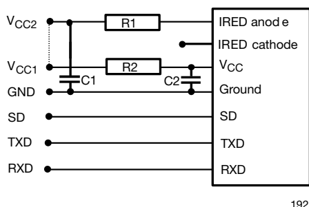
Fig. 1 - Recommended Application Circuit
