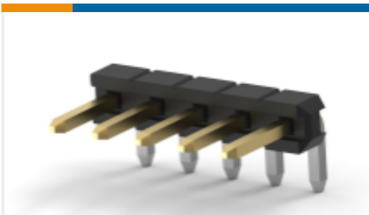
TE Part #2842124-5 5P,2MM,BRK HDR,SRRT,2.8,0.76AU, BOX
