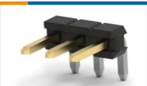
TE Part #2842116-4 4P,2MM,BRK HDR,SRRT,2.8,0.76AU,TB W/CAP
