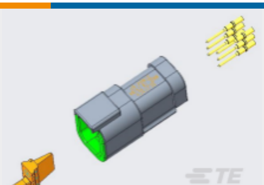
TE Part #DTM04-6P-COMplete DTM04-6P W/ WEDGELOCK AND TERMINALS
