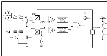
Figure 14 Boost Follower
