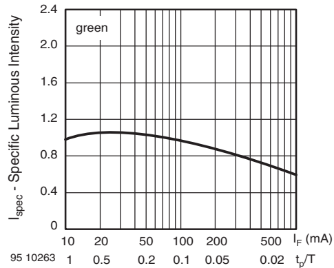
Fig. 20 - Specific Luminous Intensity vs. Forward Current
