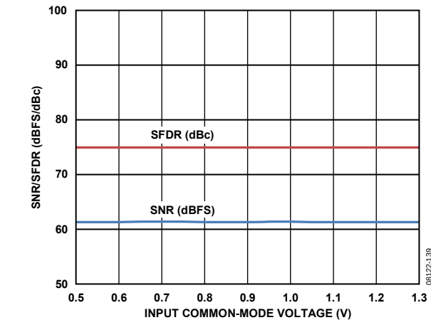
Figure 39. SNR/SFDR vs. Input Common-Mode Voltage, f_{IN} = 32.1 MHz, f_s = 80 MSPS
