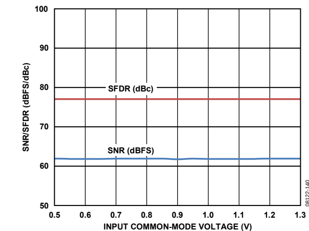
Figure 40. SNR/SFDR vs. Input Common-Mode Voltage, f_{IN} = 10.3 MHz, f_s = 20 MSPS
