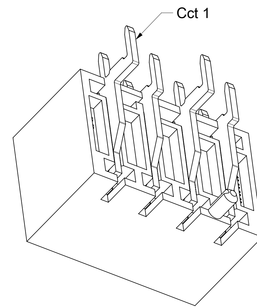
P.C.B. OPTION "A"
