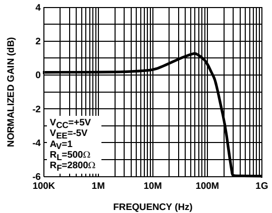
FIGURE 2. FREQUENCY RESPONSE
