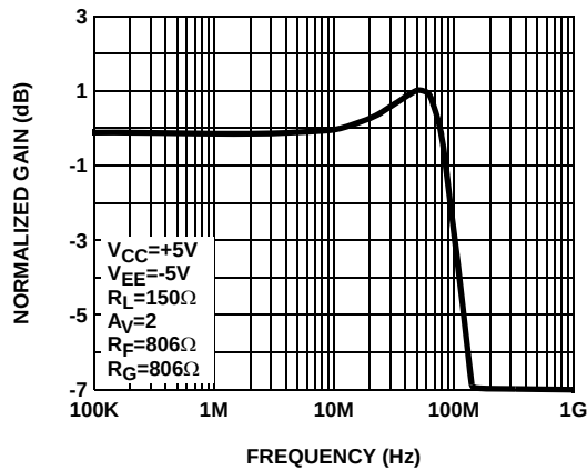
FIGURE 1. FREQUENCY RESPONSE
