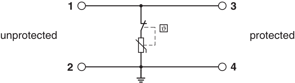
Circuit diagram
