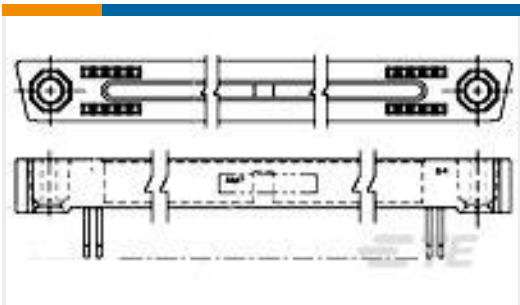
TE Part #530746-1 MINI-BOX RCPT ASSY 128 POS
