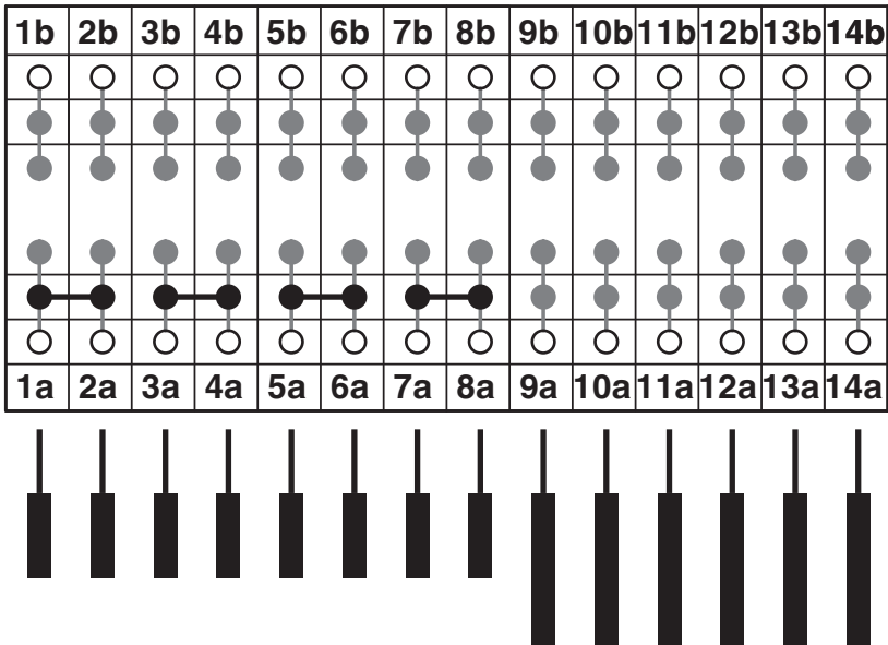
Circuit diagram
