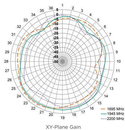
XY-Plane Gain
