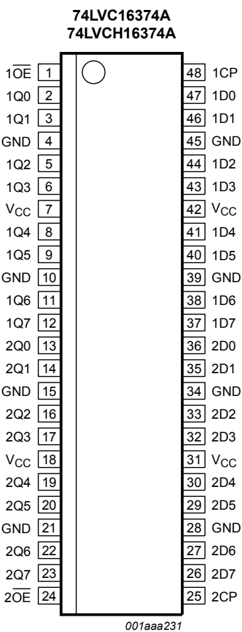
Fig. 5. Pin configuration SOT370-1 (SSOP48) and SOT362-1 (TSSOP48)
