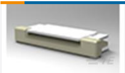
TE Part #1-1734839-6 FPC CONN. 0.5MM PITCH T/C,16P
