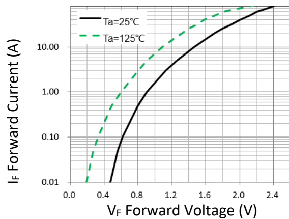
Figure 1. Forward Characteristic(typ.)
