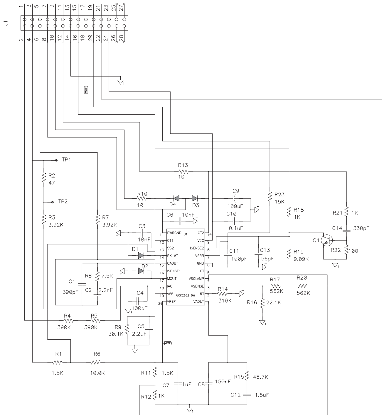
Figure 3. Daughter Board
