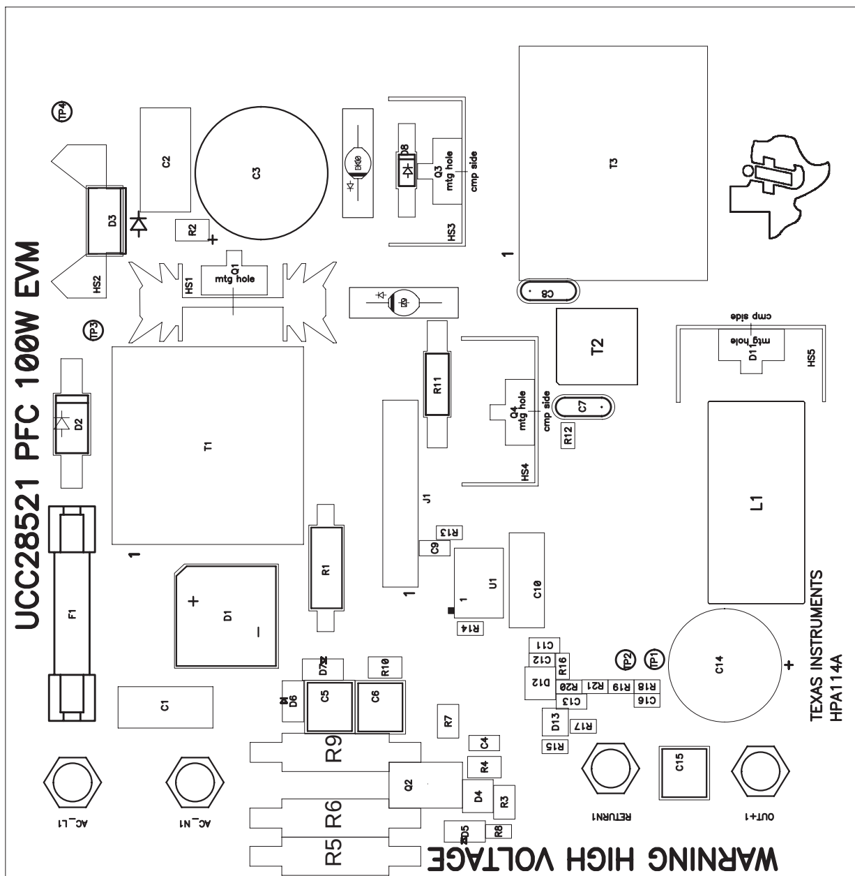
Figure 4. Mother Board
