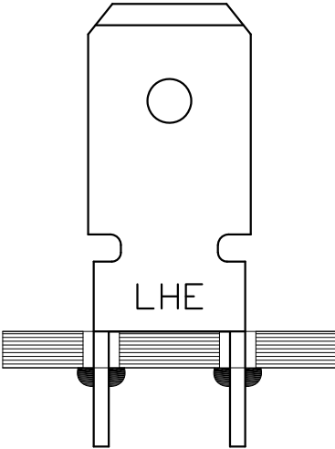
SOLDERING GRAPHIC FOR REFERENCE ONLY
