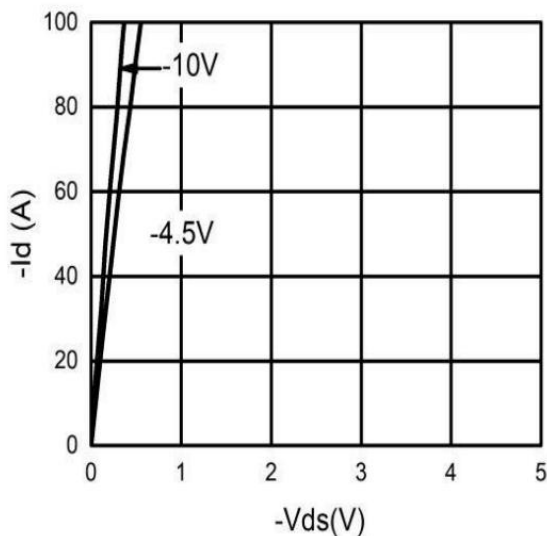
Figure 1. Output Characteristics
