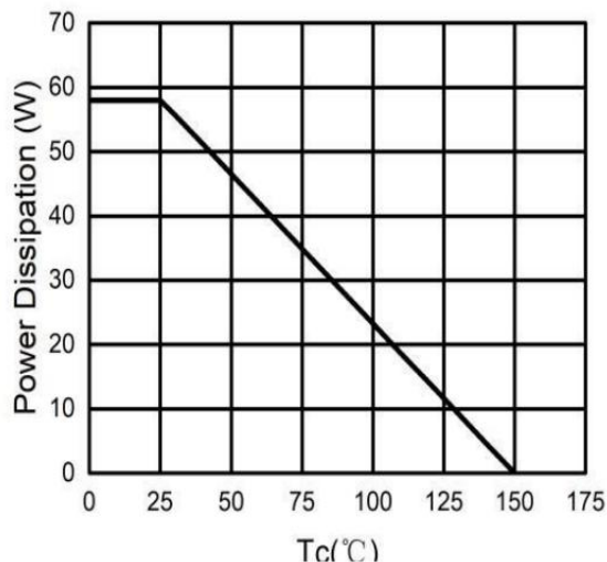
Figure 3. Power Dissipation
