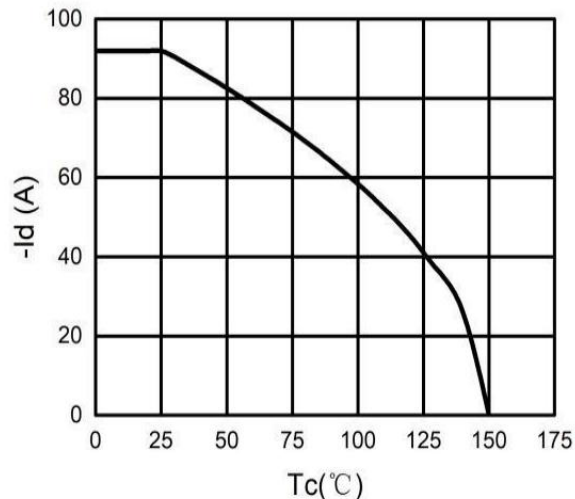
Figure 4. Drain Current
