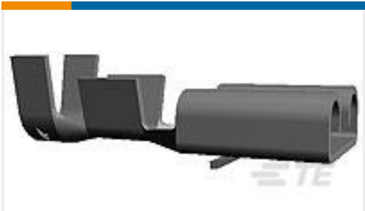
TE Part #5-160558-2 FF 250 REC 0.5-1.5MM2 TPBR
