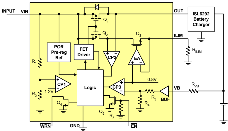
FIGURE 1. BLOCK DIAGRAM
