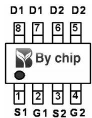
Pin Assignment
