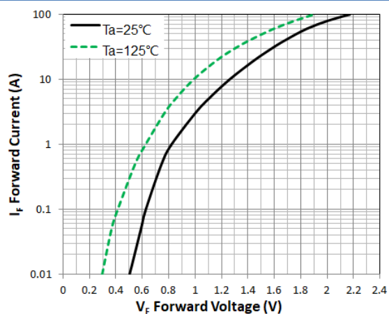
Figure 1. Forward Characteristic(typ.)
