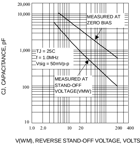
Fig. 4-TYPICAL JUNCTION CAPACITANCE
