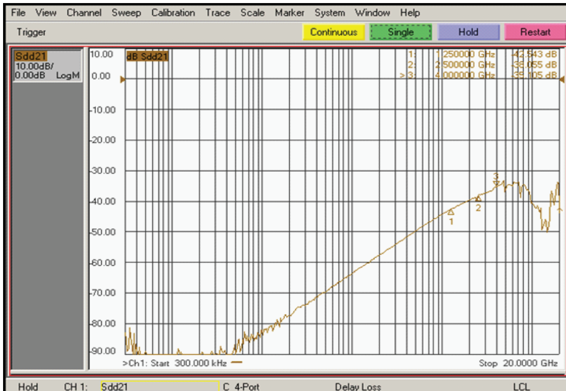
Differential Crosstalk
