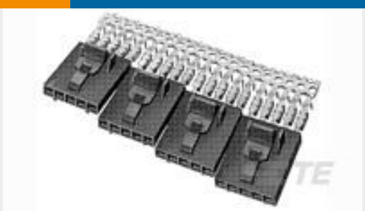
TE Part #5-103958-1 10X2 MTE RPT SR LATCH .100CL
