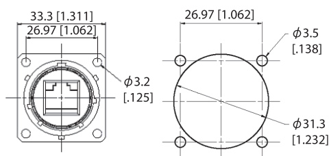
Panel Drilling
